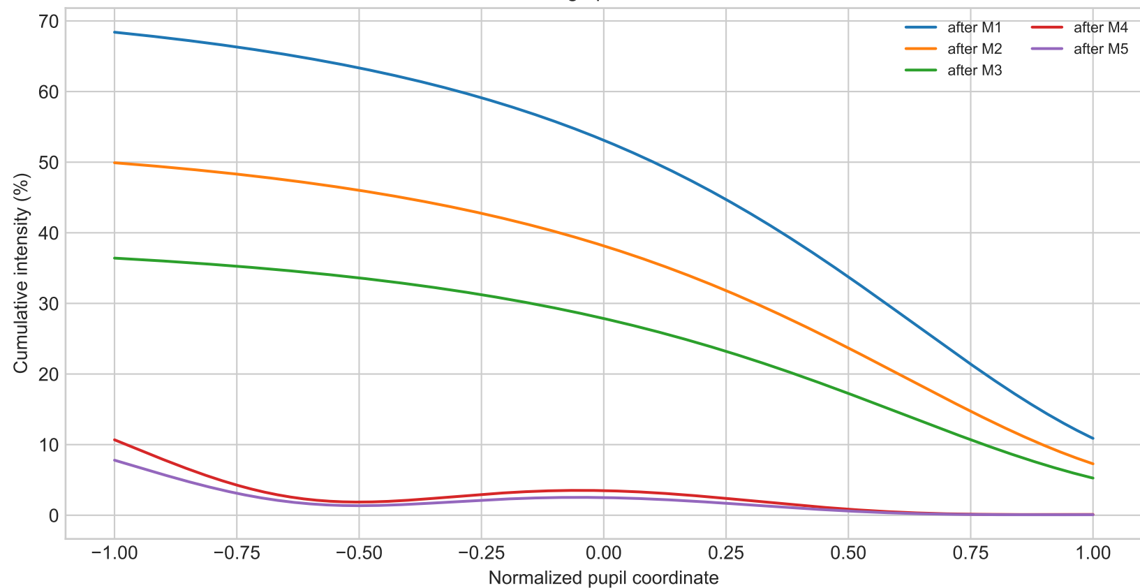
Estimated coating apodization at 13.5 nm
